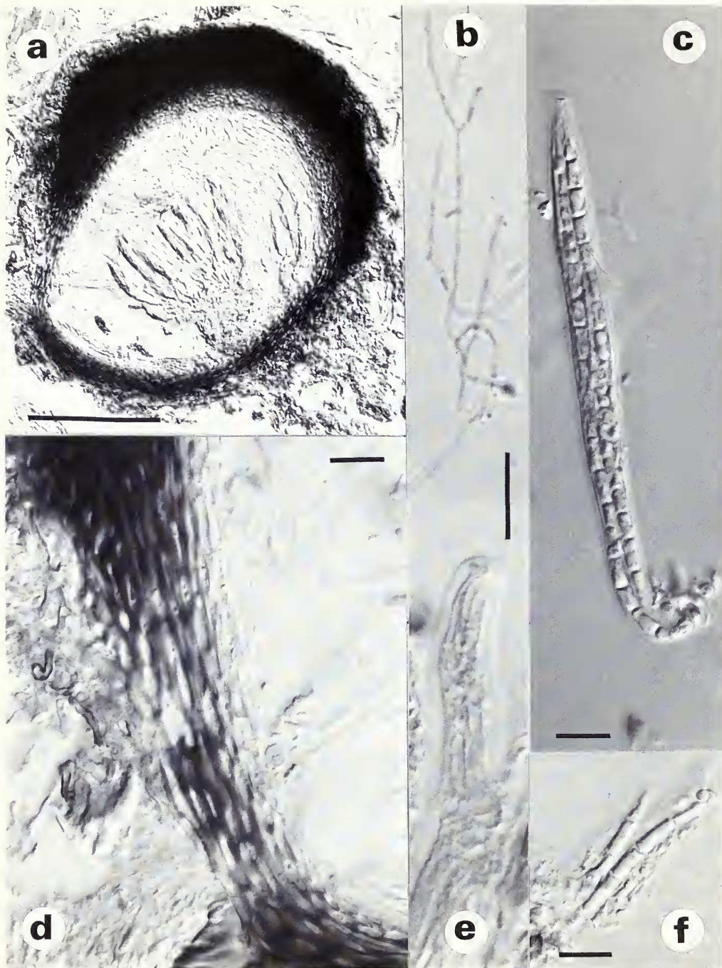
Fig. 66 Porina borrieri (Trevisan) D. Hawksw. & James (Concarneau–holotype of Verrucaria longispora ) (a) Vertical section of ascoma; scale = 100 \mu\text{m} ; (b) Branching paraphyses; (c) Ascus and ascospores; (d) Detail of exciple: textura porrecta; (e) Detail of ascus apex; (f) Ascospores; scale = 10 \mu\text{m} .
